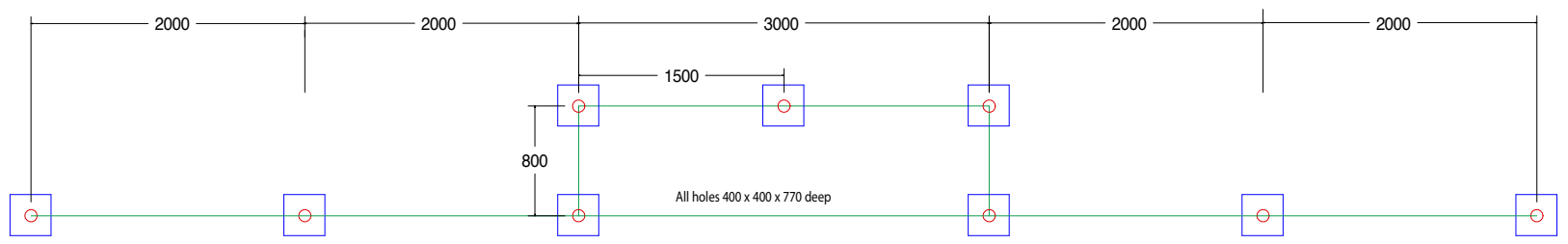
HOLE PLAN FOR GOODISON SPORTS GOAL
